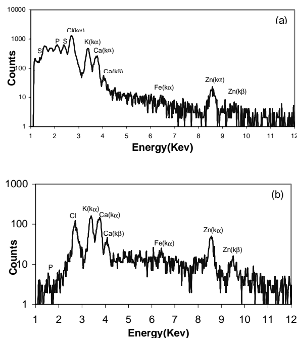
Figure 1. Typical spectrum for malignant type of human breast tissue, (a) for low Z elements (without absorber filter) and (b) for high Z elements with 175μ mylar absorber.
