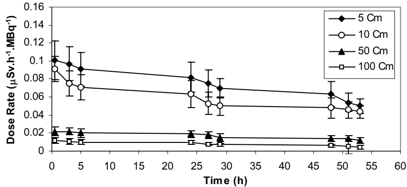
Figure 1. Mean external dose rate per unit activity of 201 Tl as a function of time.
